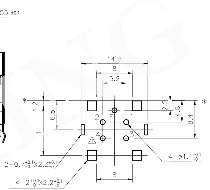
HOLE LAYOUT REFERENCE TOLERANCE : ±0.1 (BOTTOM VIEW)
