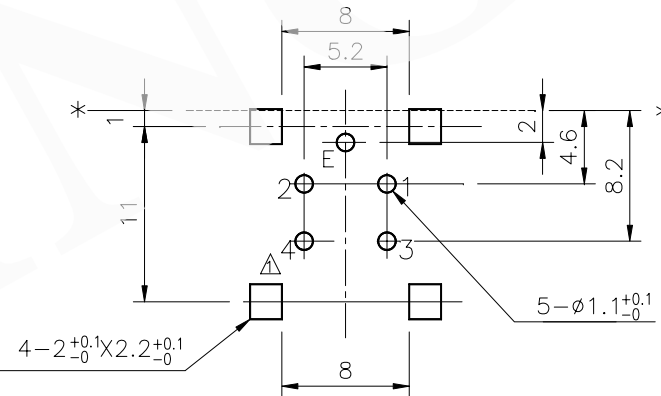
HOLE LAYOUT REFERENCE TOLERANCE : ±0.1 (BOTTOM VIEW)
