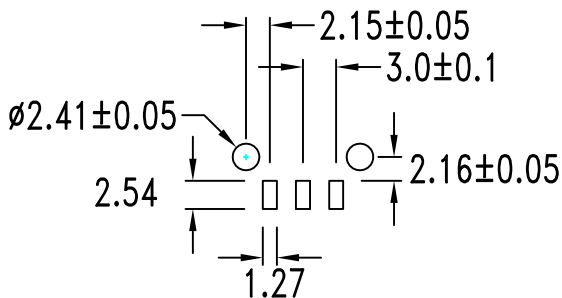
PCB Layout: Component side
