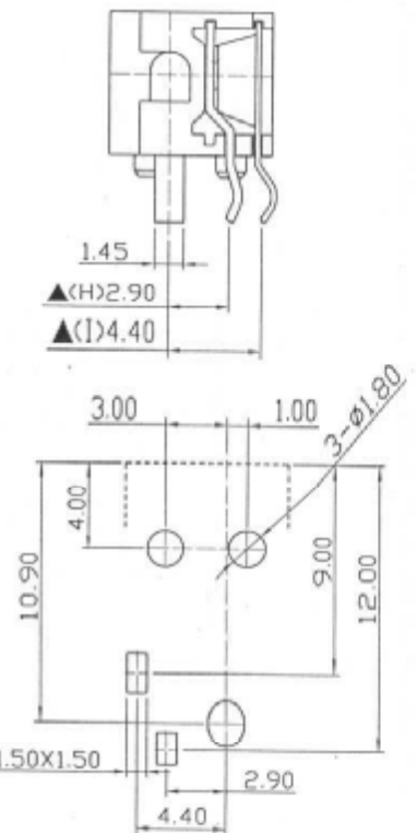
Pin Hole Layout (Jack Bottom View)
