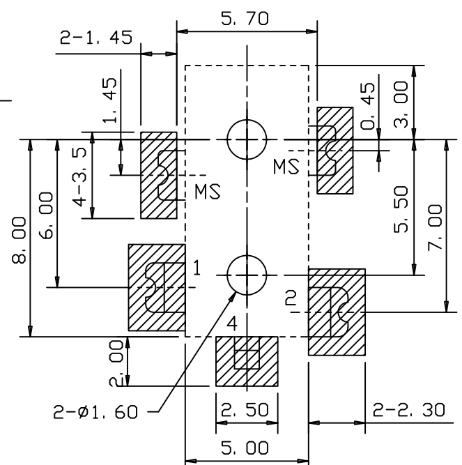
Recommended Pads Layout <TOP VIEW>
