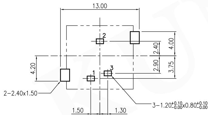
PCB Layout Dimension (Tolerance:±0.10) (Recommend min. Dimension)(Bottom View)
