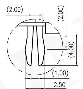
Detail A Scale:2:1 Terminal No.1,2,3
