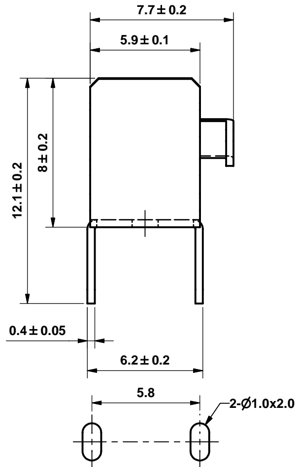
MOUNTING HOLES
