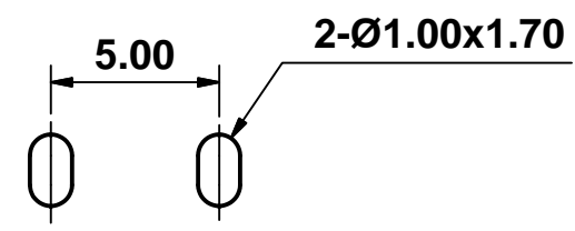
MOUNTING HOLES
