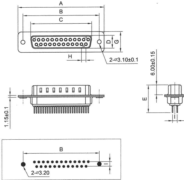
P.C. BOARD LAYOUT
