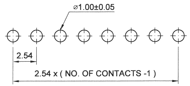
RECOMMENDED P.C. BOARD HOLE DIMM.
