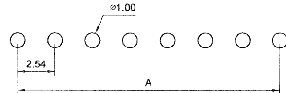
RECOMMENDED P.C. BOARD HOLE DIMM.
