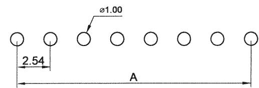
RECOMMENDED P.C. BOARD HOLE DIMM.
