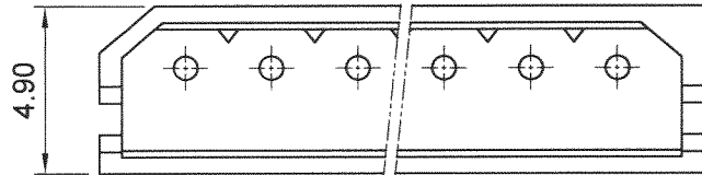
P.C.B LAYOUT COMPONENT SIDE
