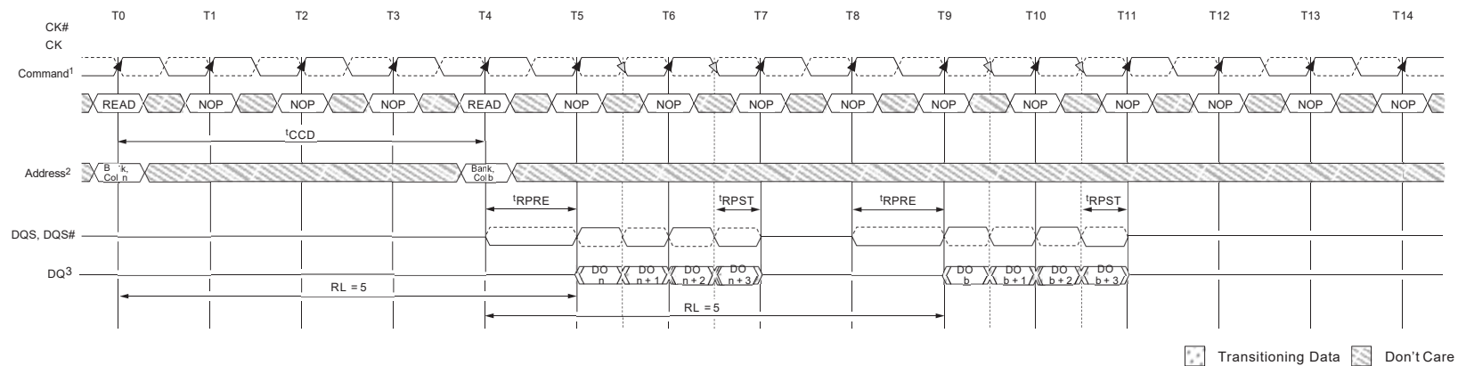
Figure 57 : Consecutive READ Bursts (BC4)
