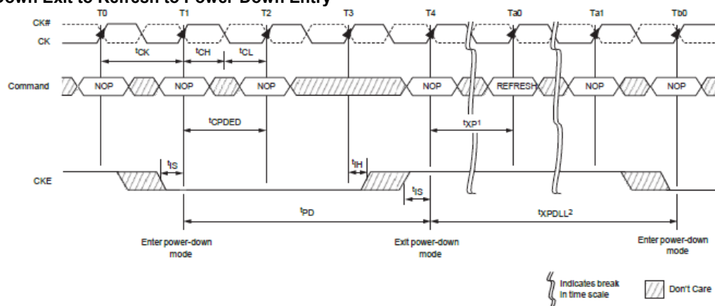
Figure 94 : Power-Down Exit to Refresh to Power-Down Entry
