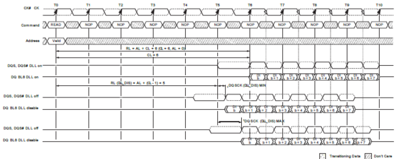
Figure 32: DLL Disable tDQSCK
