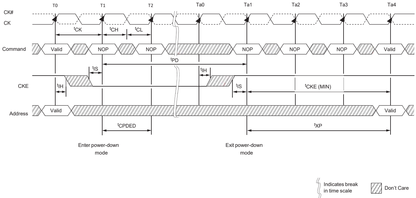
Figure 84 : Active Power-Down Entry and Exit
