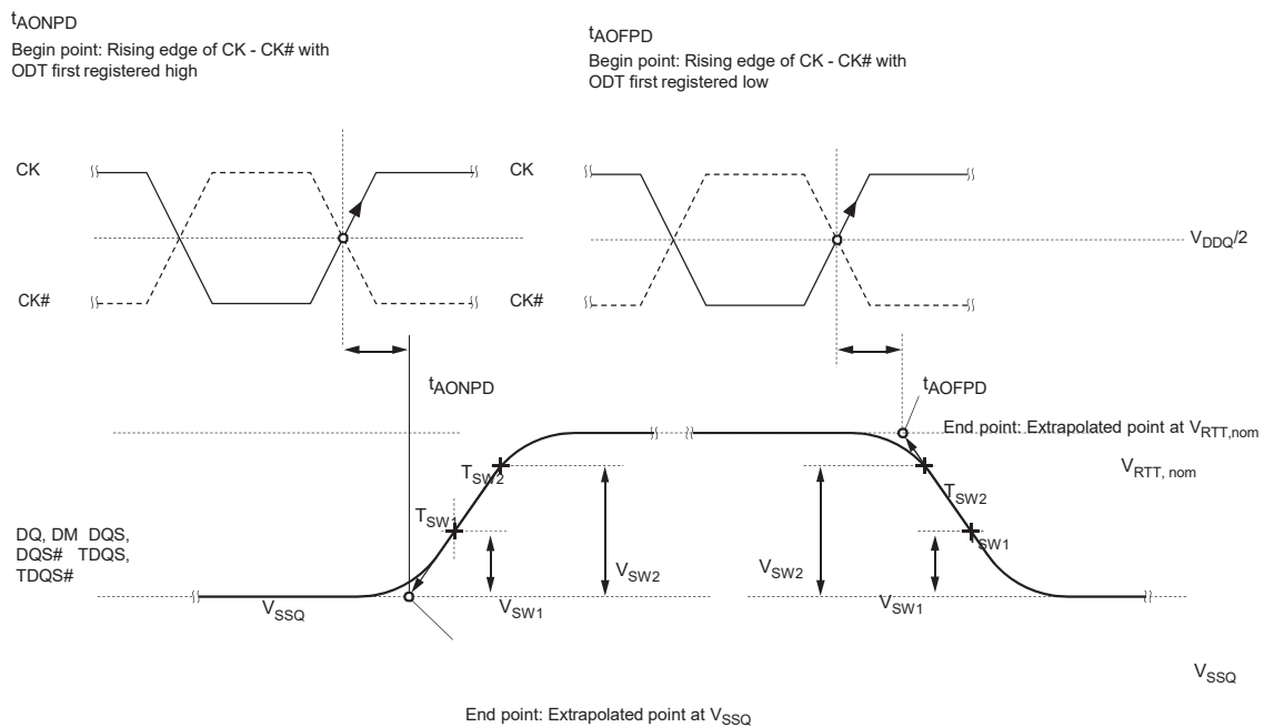
Figure 13: tAONPD and tAOFPD Definitions
