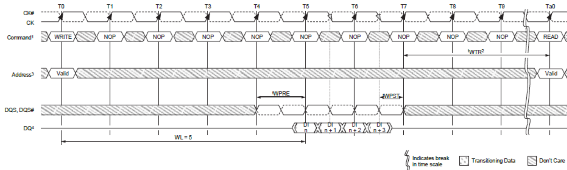
Figure 77 : WRITE to READ (BC4 Mode Register Setting)
