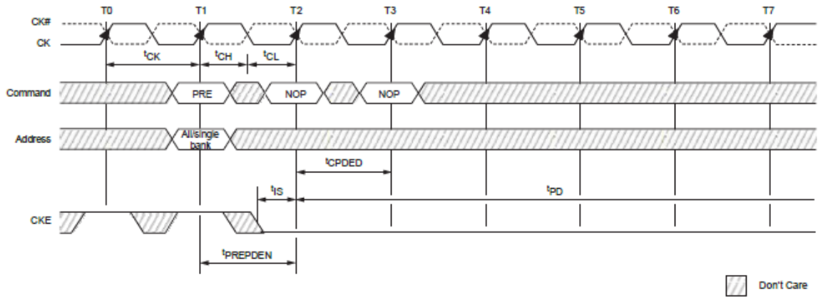
Figure 93 : MRS Command to Power-Down Entry
