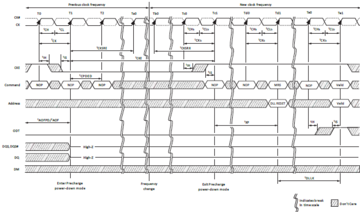
Figure 33: Change Frequency During Precharge Power-Down
