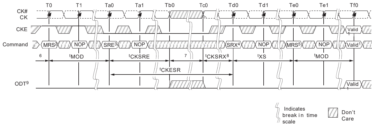
Figure 30: DLL Enable Mode to DLL Disable Mode
