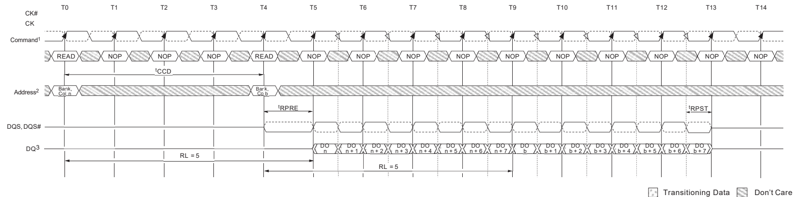
Figure 56 : Consecutive READ Bursts (BL8)
