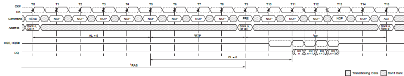
Figure 63 : READ to PRECHARGE (AL = 5, CL = 6)
