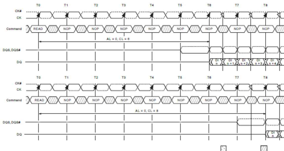
Figure 41 : READ Latency
