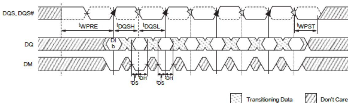
Figure 82 : Data Input Timing
