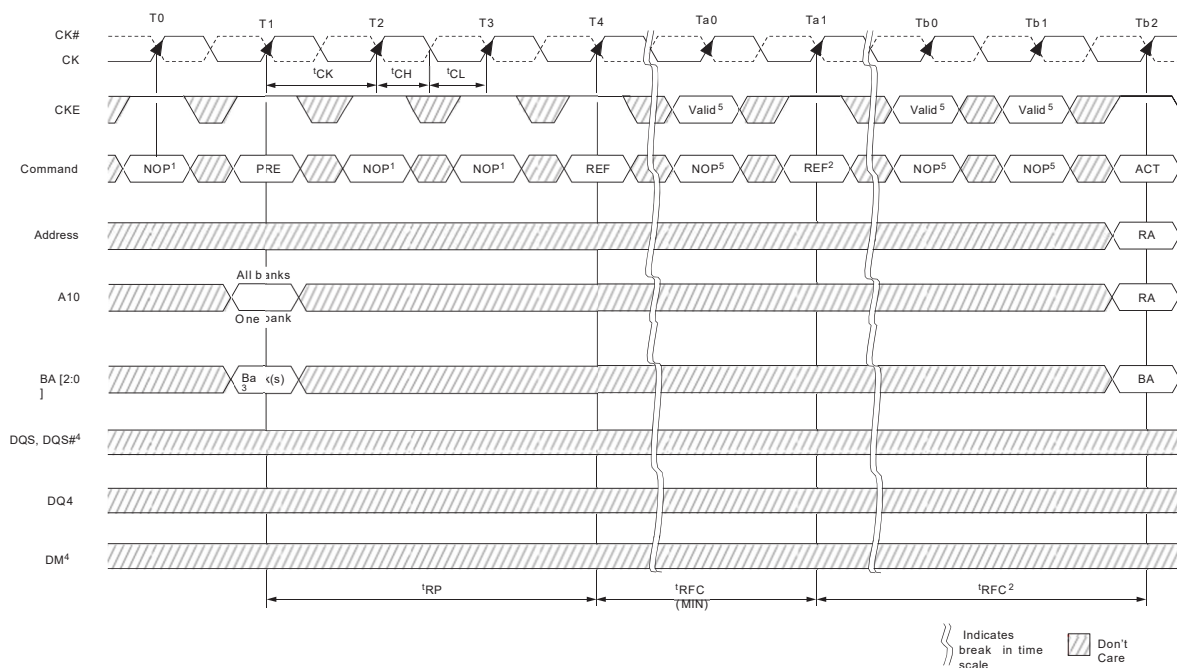
Figure 29: Refresh Mode
