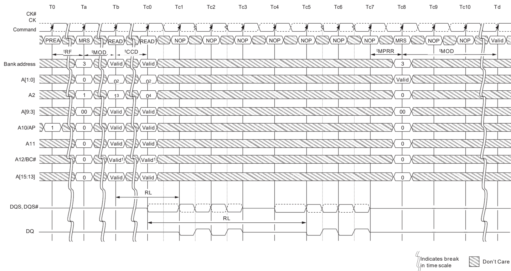
Figure 51 : MPR System Read Calibration with BC4: Upper Nibble, Then Lower Nibble
