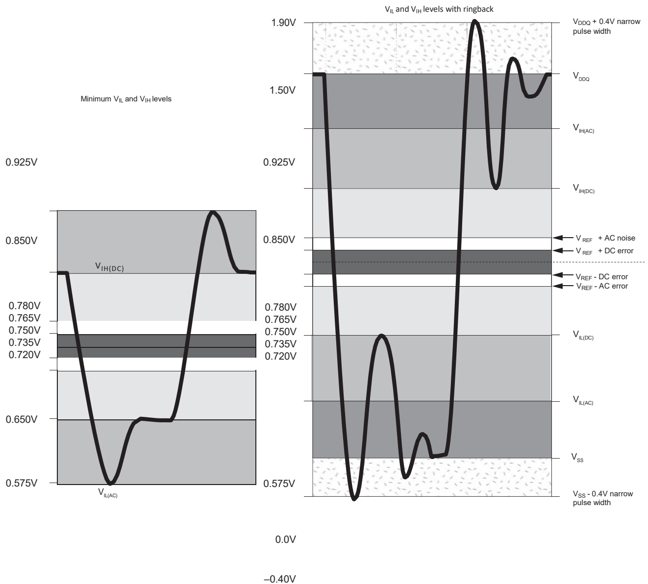
Figure 2: Input Signal
