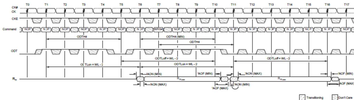
Figure 103 : Synchronous ODT (BC4)
