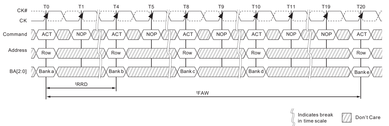
Figure 54 : Example: tFAW
