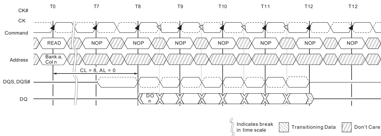
Figure 55 : READ Latency
