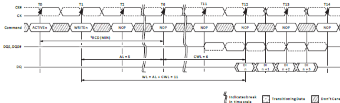
Figure 45 : CAS Write Latency
