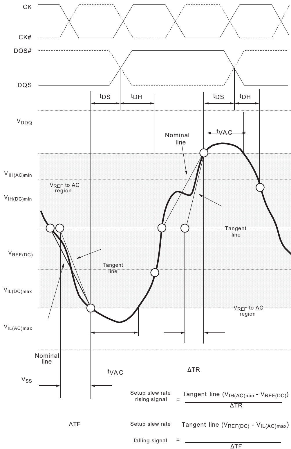
Figure 27: Tangent Line for tDS (DQ – Strobe)
