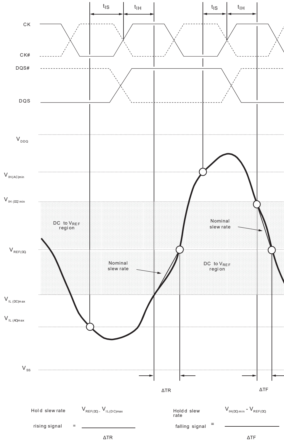
Figure 22: Nominal Slew Rate for t IH (Command and Address – Clock)
