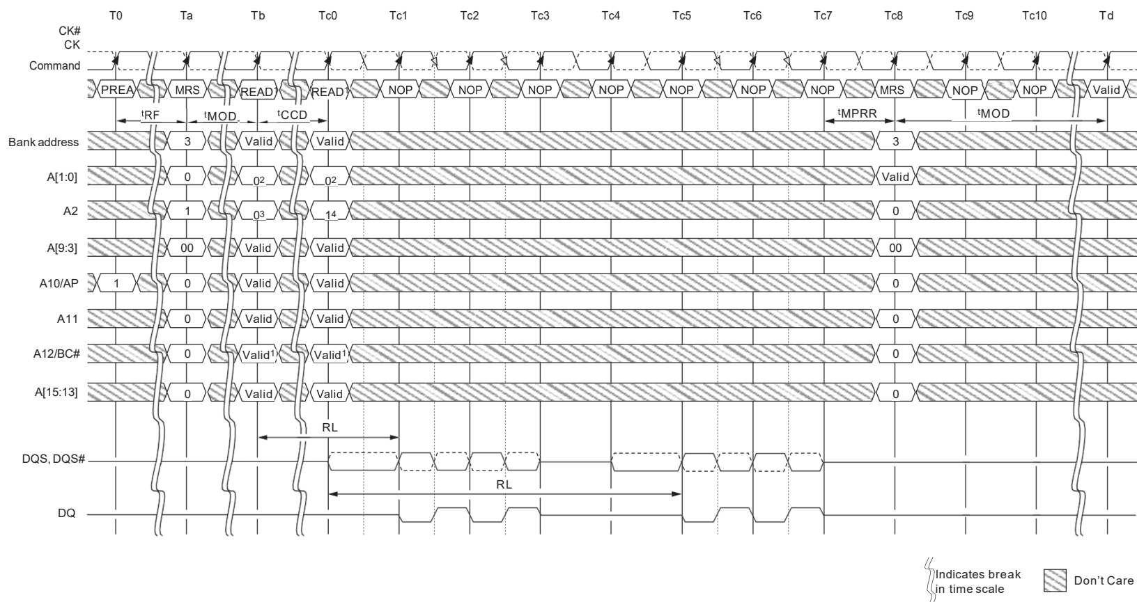
Figure 50 : MPR System Read Calibration with BC4: Lower Nibble, Then Upper Nibble
