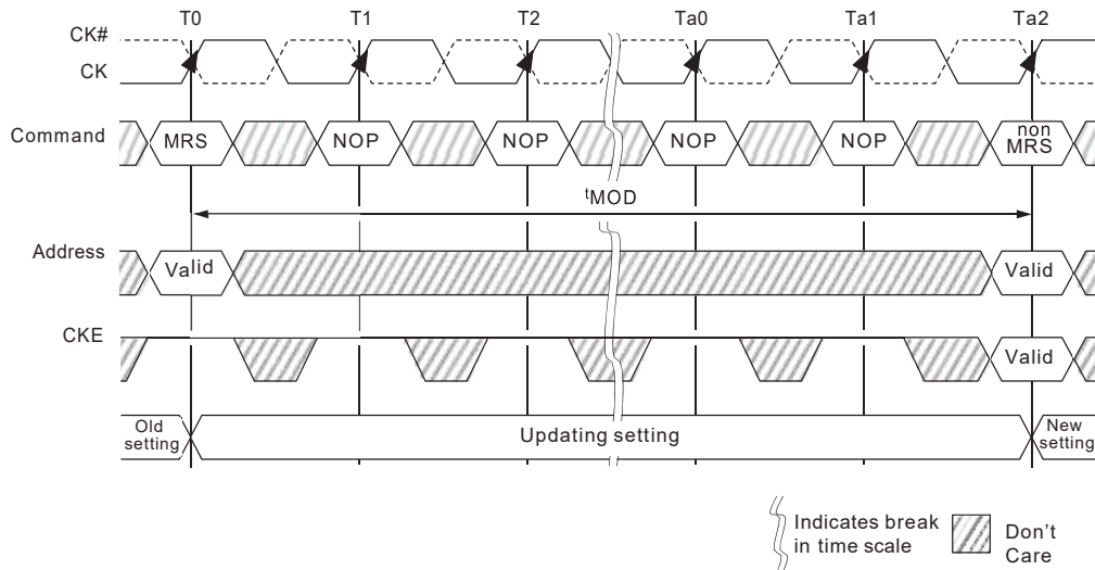
Figure 39: MRS to nonMRS Command Timing (tMOD)
