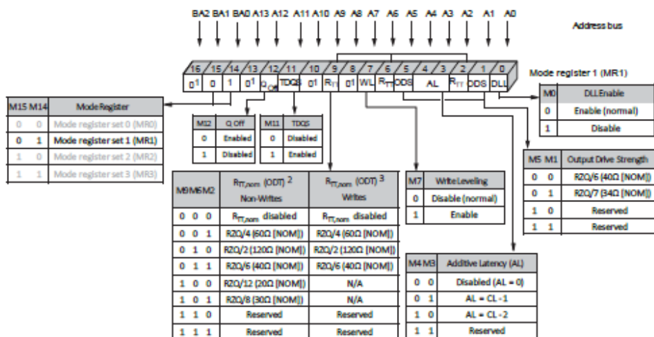
Figure 42 : Mode Register 1 (MR1) Definition
