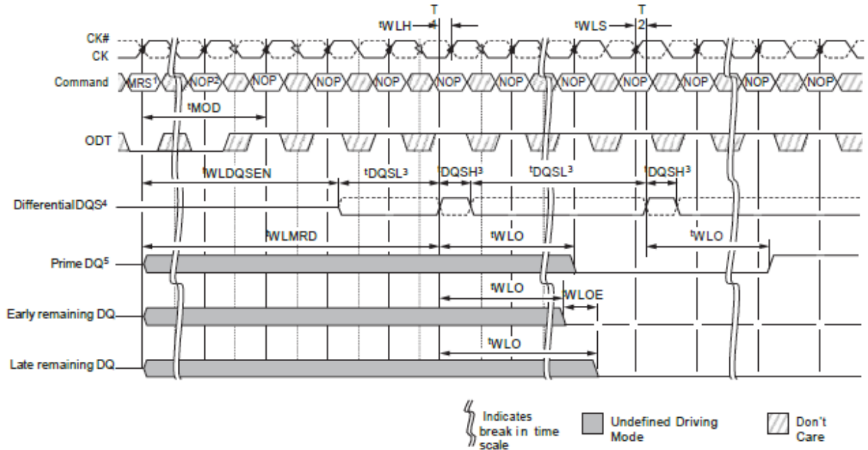
Figure 35: Write Leveling Sequence
