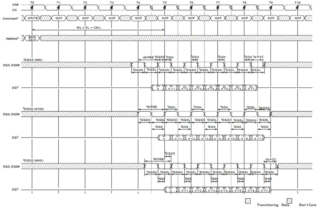
Figure 72 : WRITE Burst
