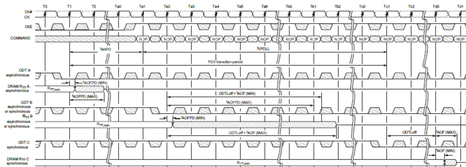
Figure 107 : Asynchronous to Synchronous Transition During Precharge Power-Down (DLL Off) Exit
