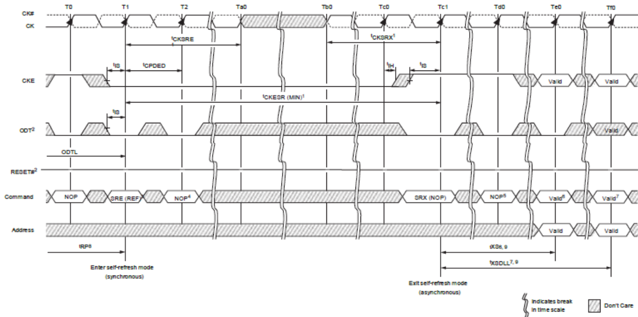
Figure 83 : Self-Refresh Entry/Exit Timing
