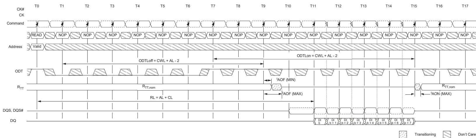
Figure 104 : ODT During READs
