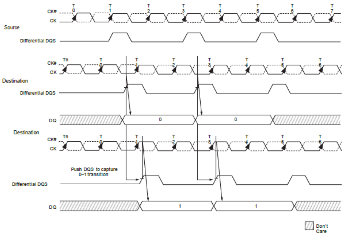
Figure 34: Write Leveling Concept
