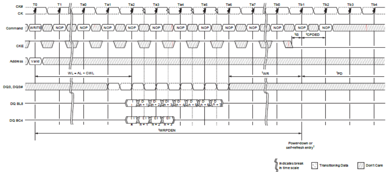
Figure 88 : Power-Down Entry After WRITE
