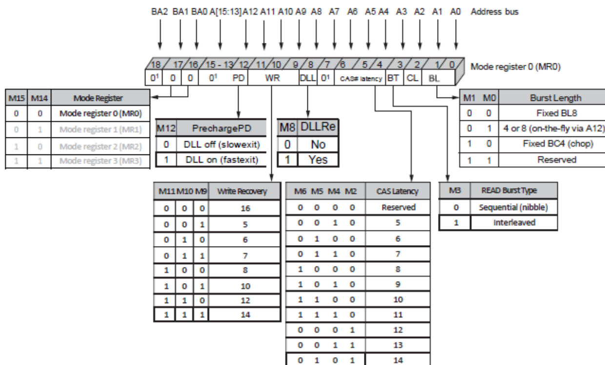
Figure 40: Mode Register 0 (MR0) Definitions
