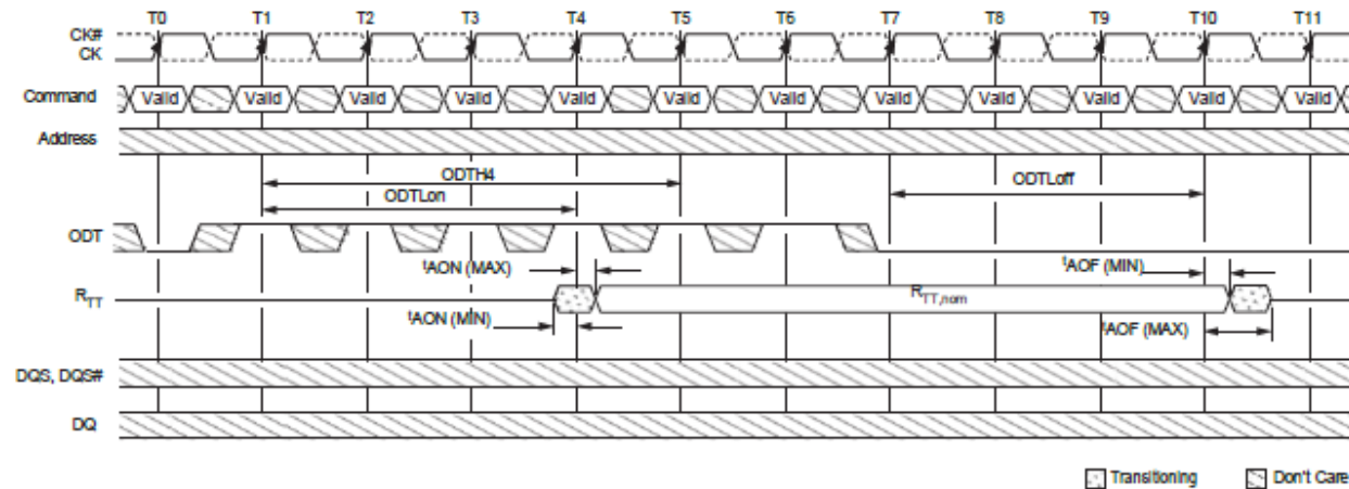
Figure 98 : Dynamic ODT: Without WRITE Command
