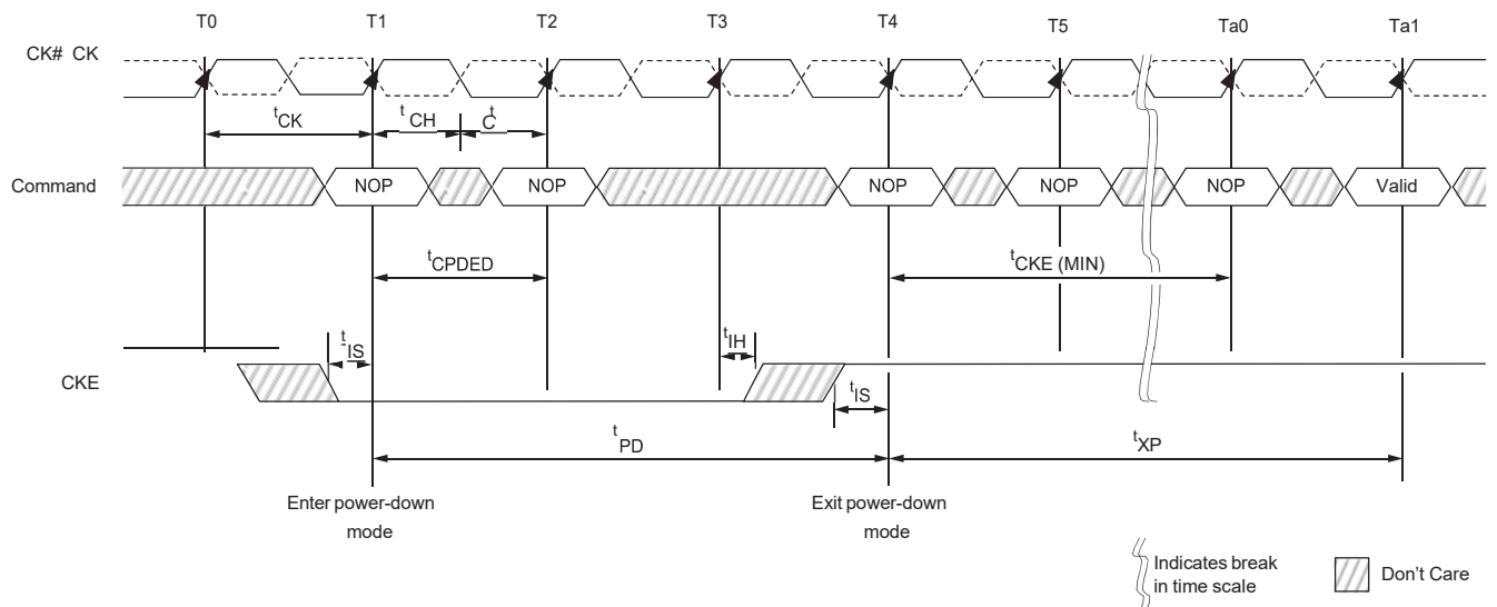
Figure 85 : Precharge Power-Down (Fast-Exit Mode) Entry and Exit
