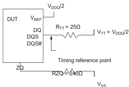
Figure 18: Reference Output Load for AC Timing and Output Slew Rate
