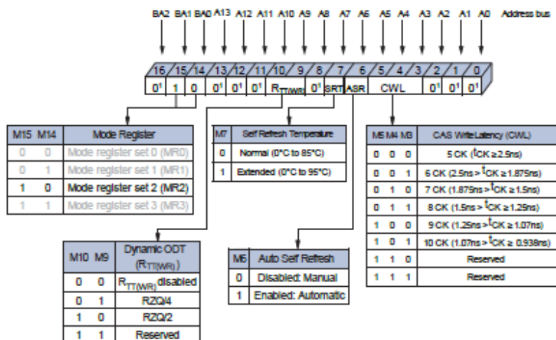
Figure 44 : Mode Register 2 (MR2) Definition
