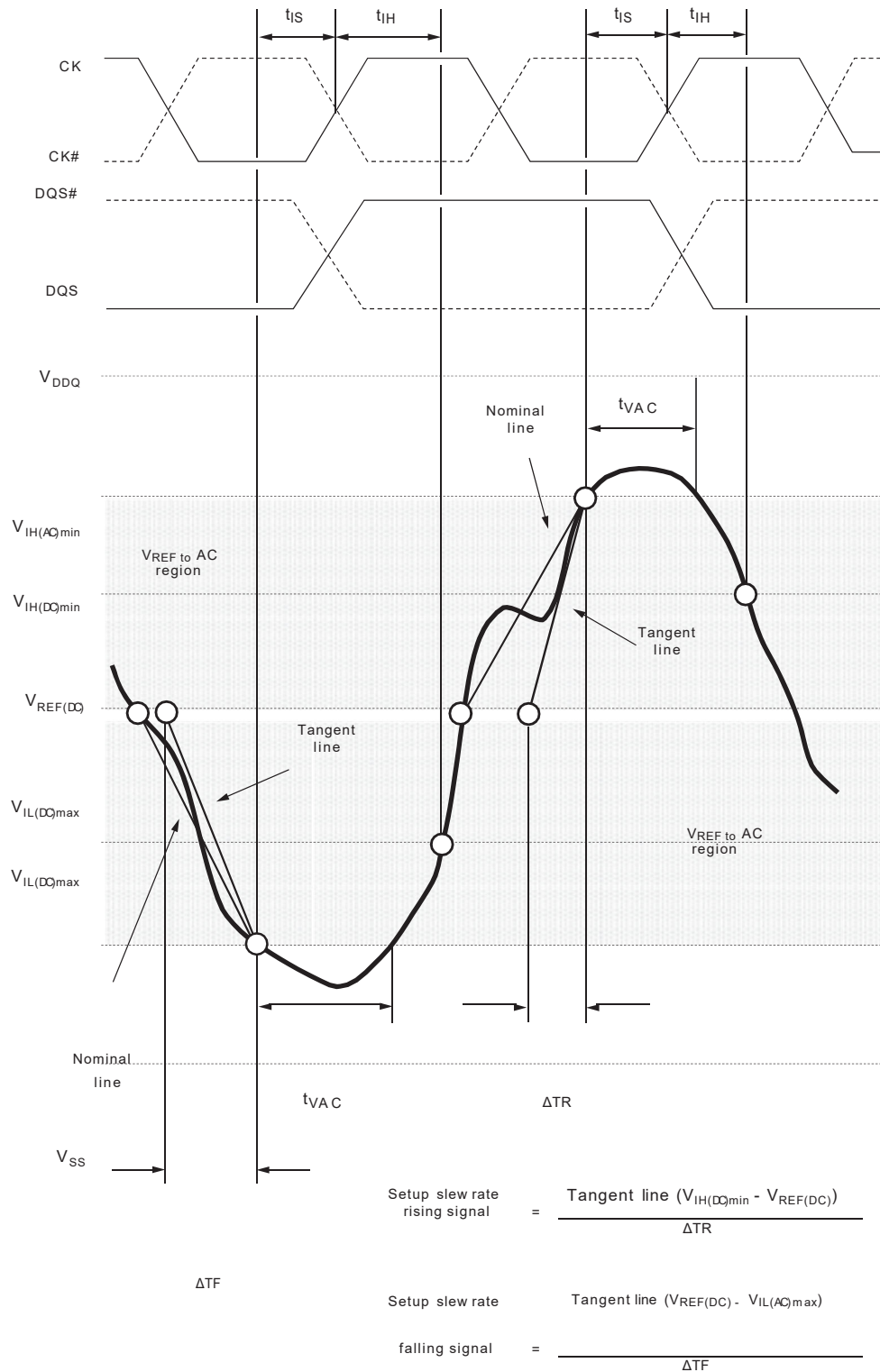
Figure 23: Tangent Line for tIS (Command and Address – Clock)
