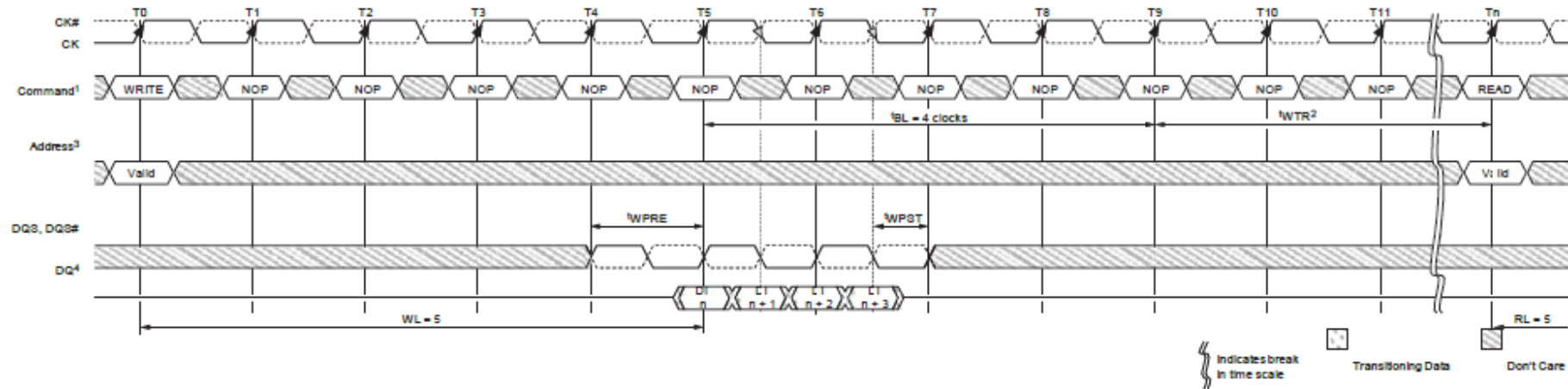
Figure 78 : WRITE (BC4 OTF) to READ (BC4 OTF)
