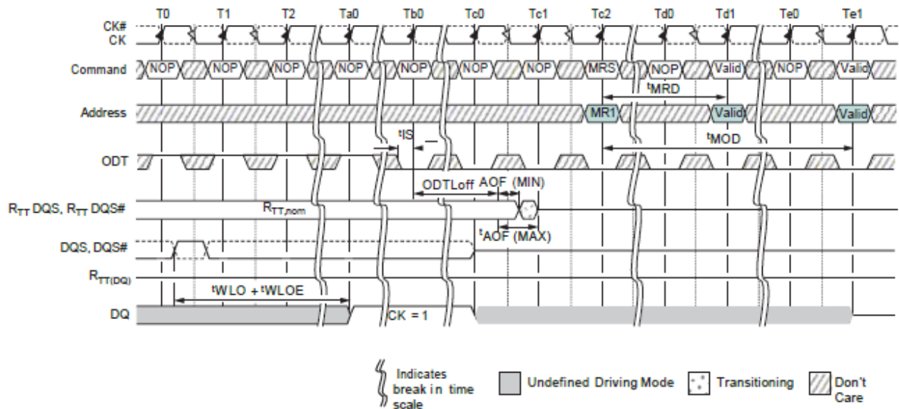
Figure 36: Write Leveling Exit Procedure
