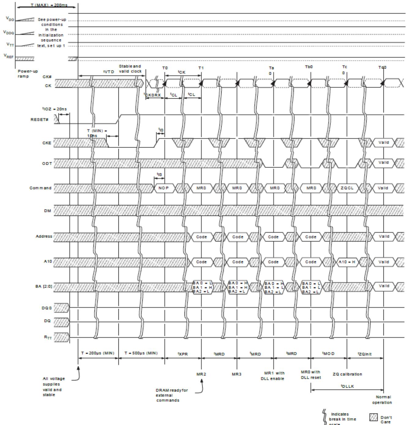
Figure 37: Initialization Sequence
