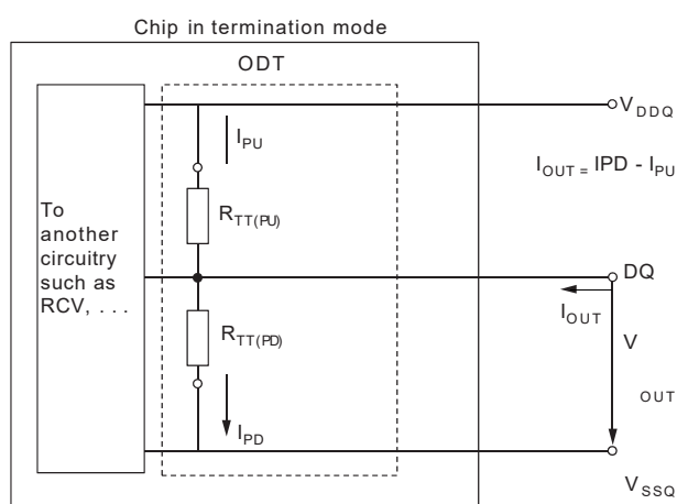
Figure 10: ODT Levels and I-V Characteristics
