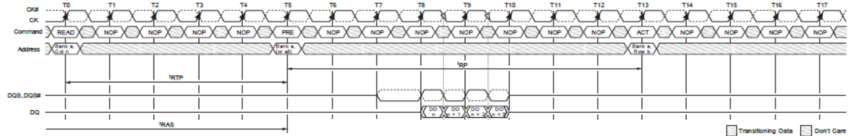
Figure 62 : READ to PRECHARGE (BC4)
