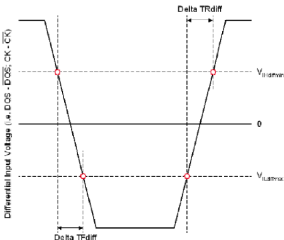
Differential Input Slew Rate Definition for \overline{DQS} , \overline{DQS} and \overline{CK} , \overline{CK}
