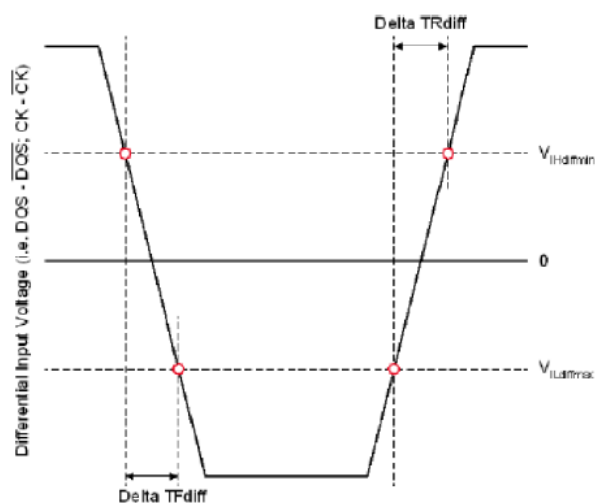
Differential Input Slew Rate Definition for DQS, \overline{DQS} and CK, \overline{CK}
