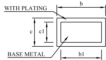
DETAIL B-B
