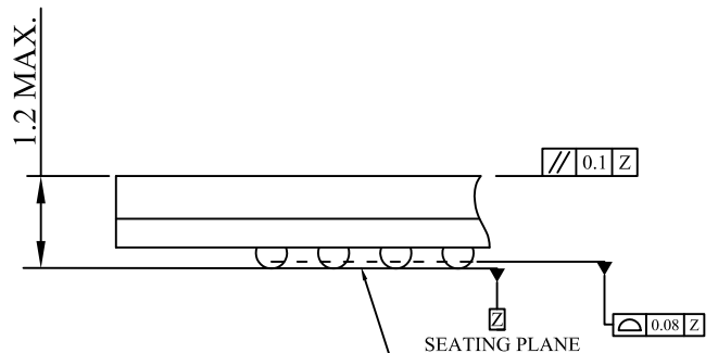
DETAIL A
