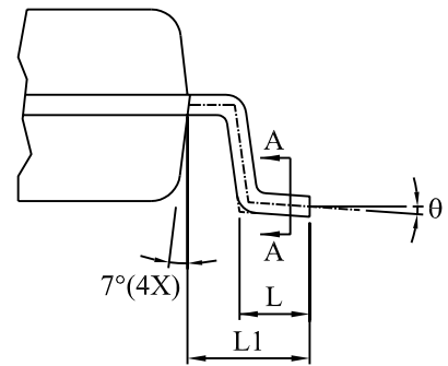
DETAIL "A" (2:1)
