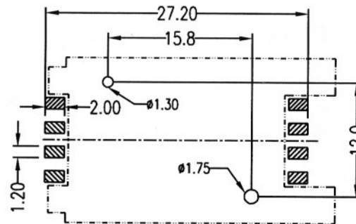
RECOMMEND P.C.B. LAYOUT TOP VIEW
